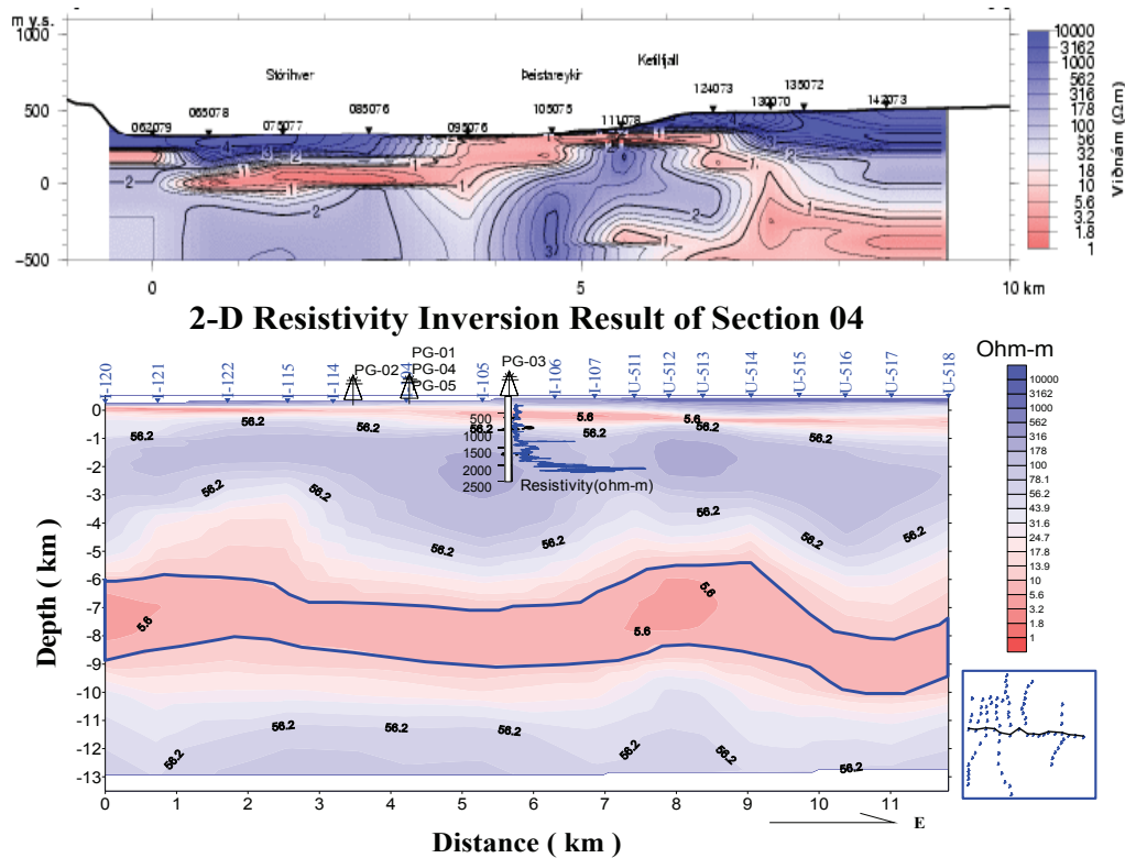
Figure 1: Top: TEM inversion result of profile 307 (from the ISOR report provided by the client); bottom: 2-D deep MT inversion section shows the striking conductor in depth around 7 km and excellent correlation to well control.
